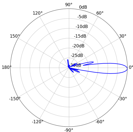
Vertical Elevation
