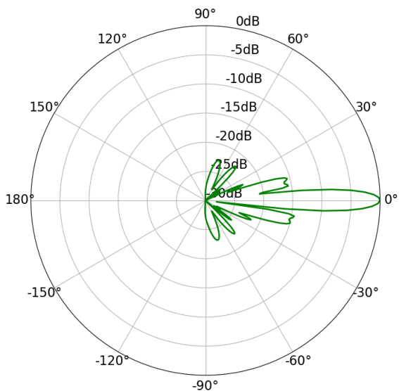
Vertical Azimuth
